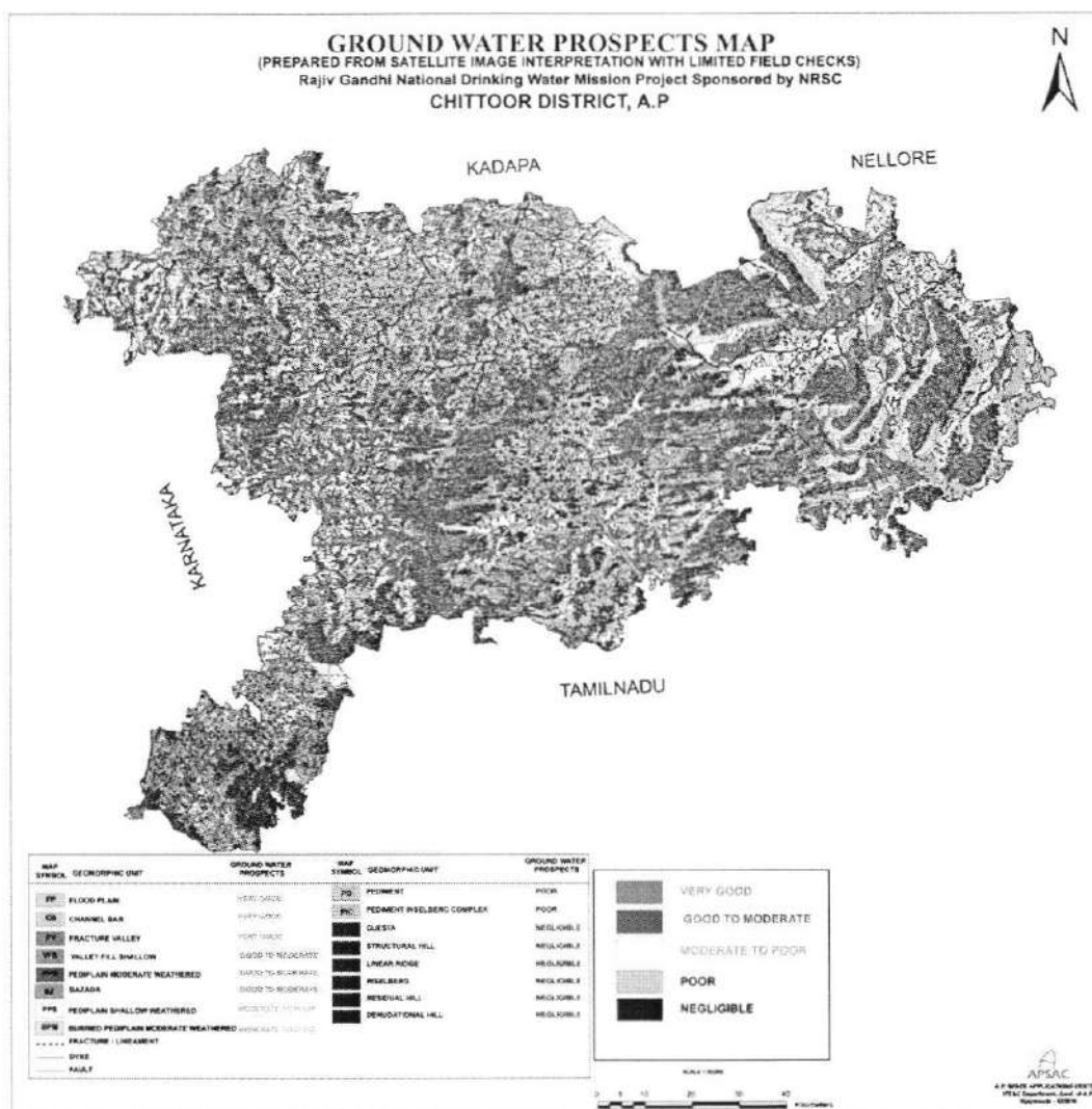
Fig:23.Groundwater prospects map of Chittoor District,A.P
